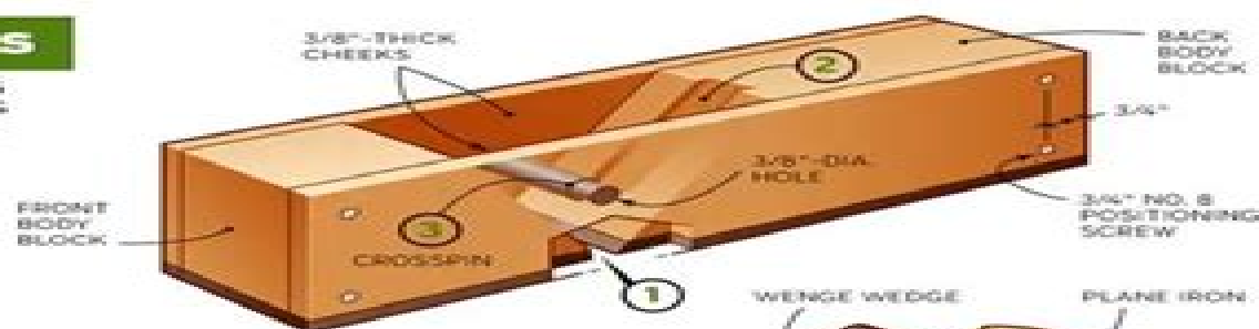
ASSEMBLED PLANE BLANK
