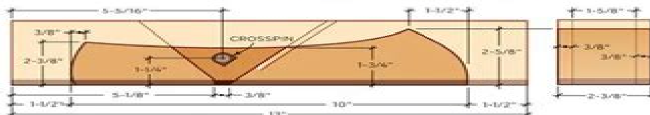
B — SMOOTH PLANE SECTION VIEW
