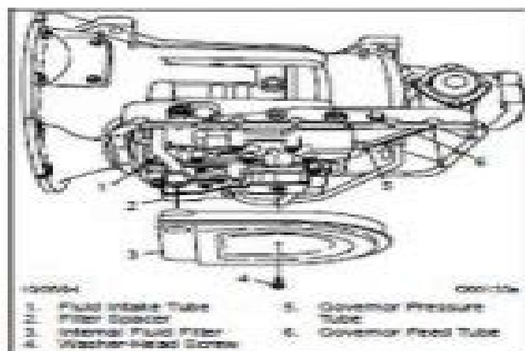
Fig. 1, AT Series Transmission Filter
