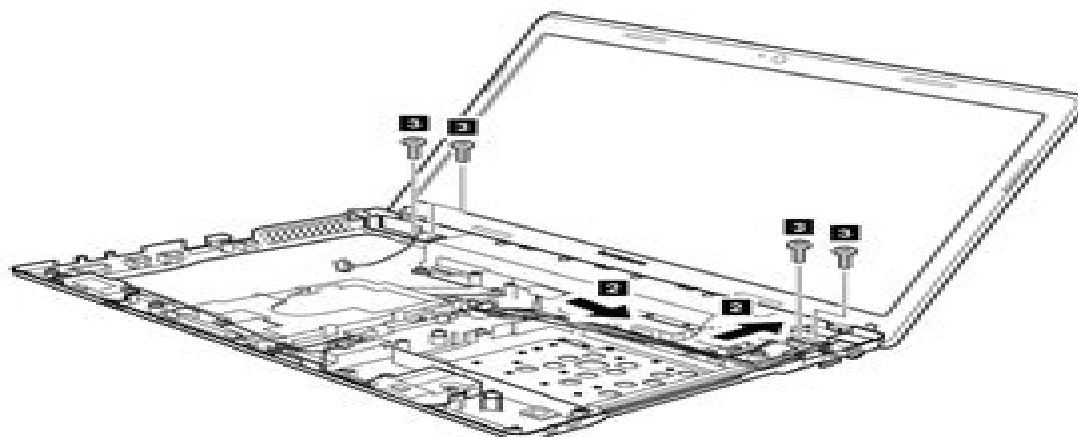
Figure 14. Removal steps of LCD unit (continued)
