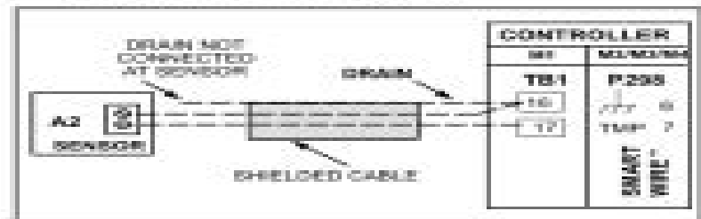
Figure 1. Sensor Wiring
