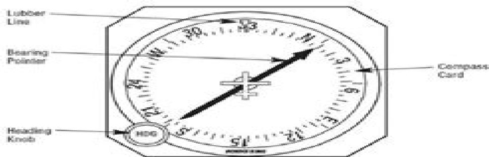
KI 227 KS 227-00 shown, non-slaved, standard KI 227-01 slaved, optional
