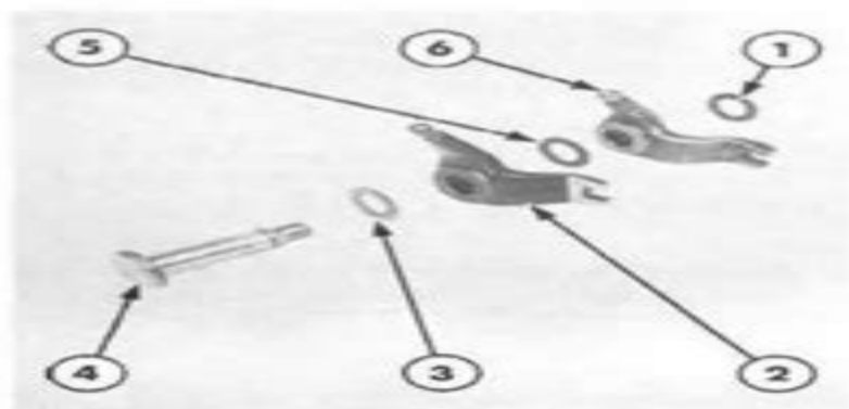
Figure 20 Bellcrank Assembly
