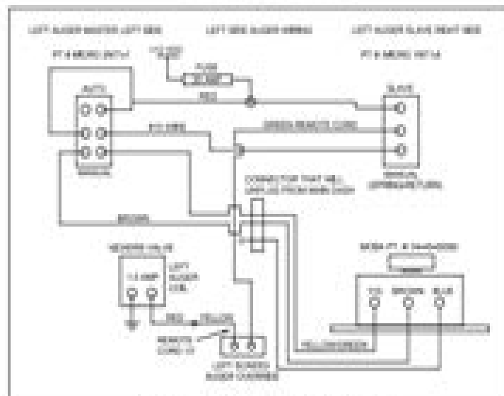
FIGURE 4-20. WEYL LEFT AUGER SWITCH WIRING
