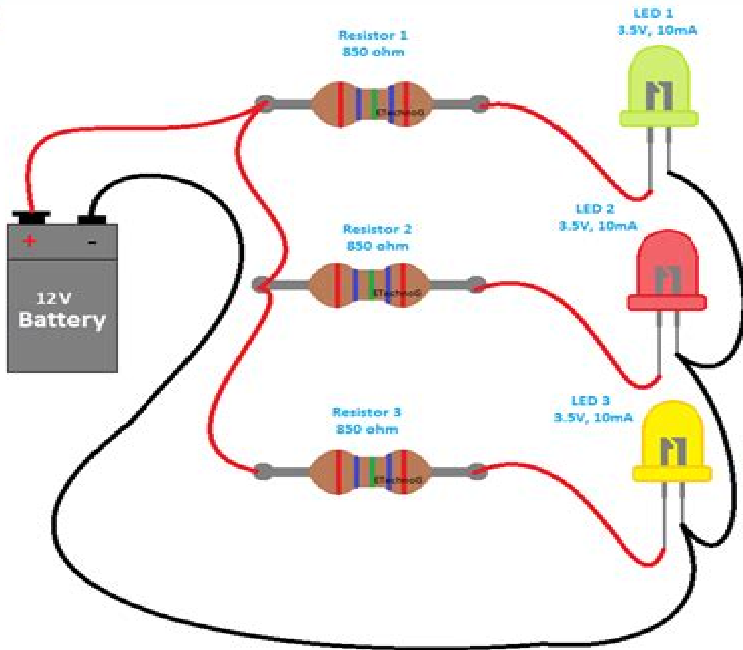
Multiple LED Wiring in Parallel Connection
