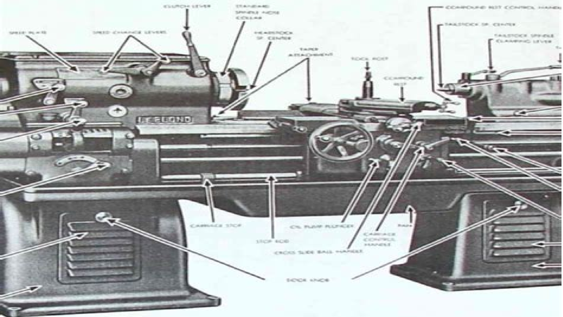
NOMENCLATURE 12" TO 18" LeBLOND ENGINE LATHES
