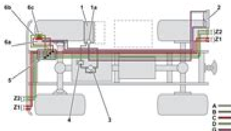
Hydraulic diagram of work hydraulics, front and rear wheel hydraulic system
