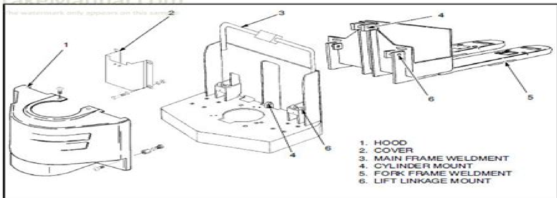
FIGURE 5 - FRAME WELDMENT - B60-80XT
