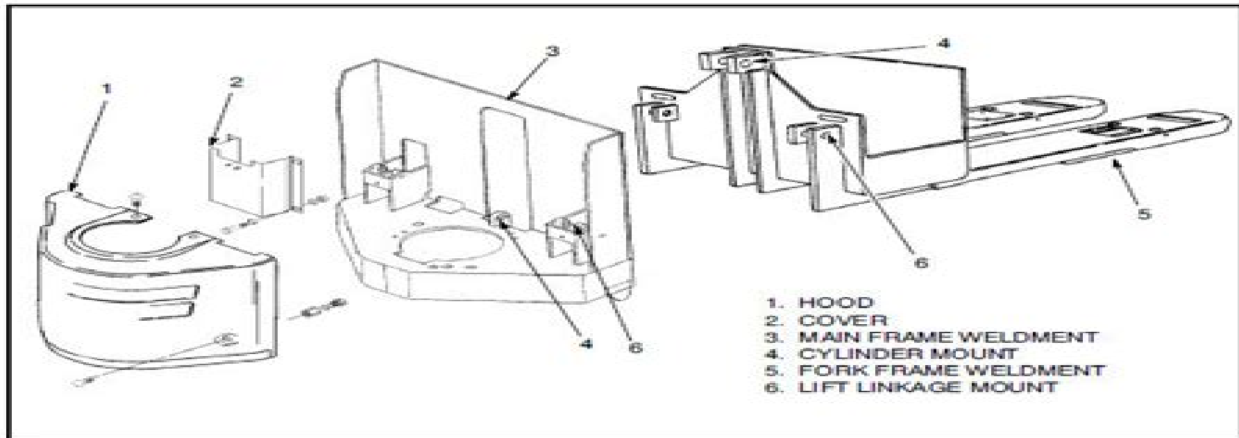
FIGURE 4 - FRAME WELDMENT - W60-80XT
