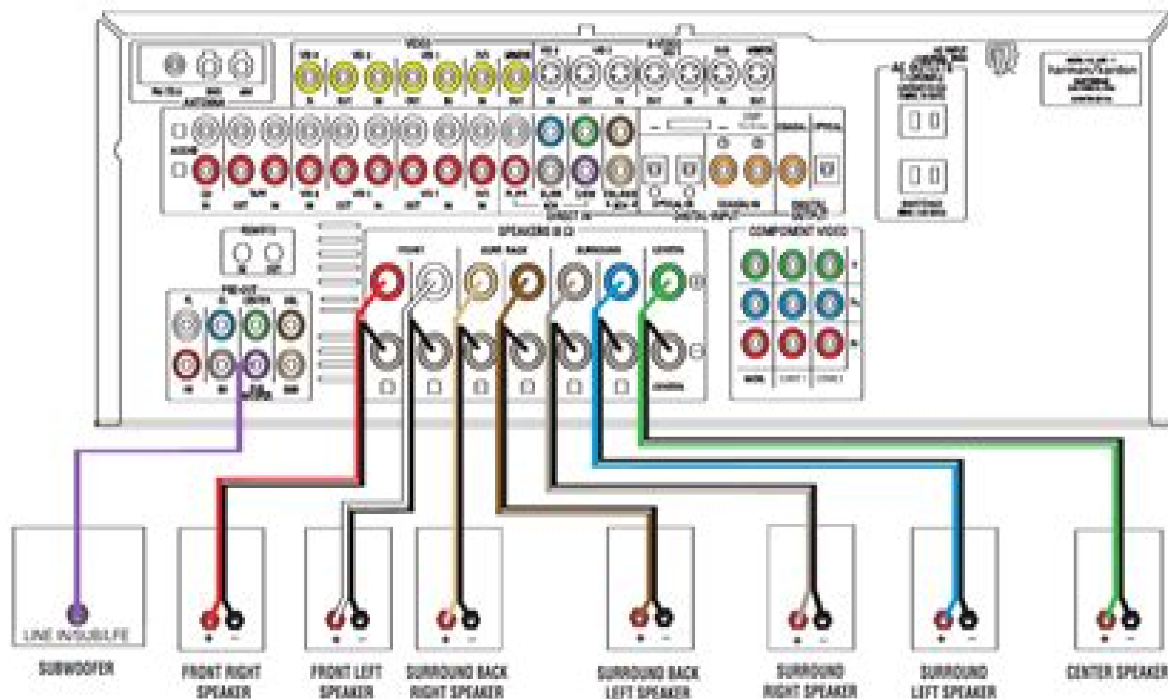
Figure 2 – Speaker Connections
