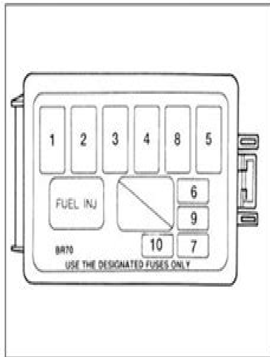
Engine compartment fuse panel (1.8 liter)
