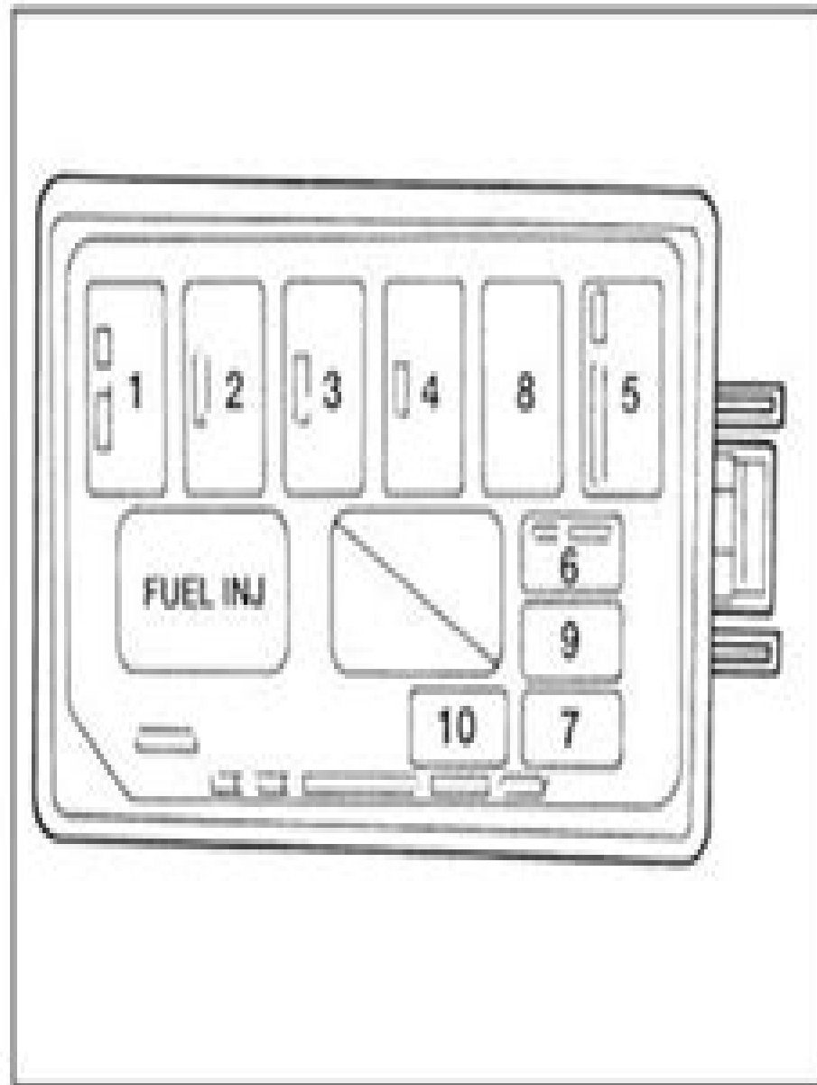
Engine compartment fuse panel (1.9 liter)
