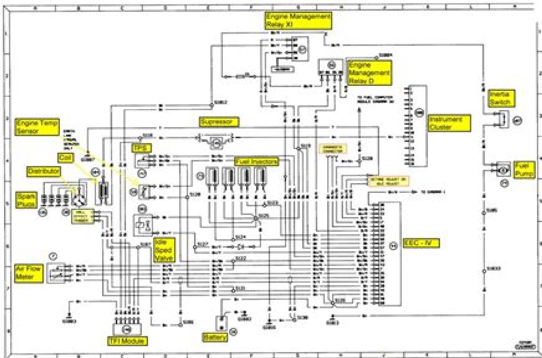
Diagram 4. 2.0i EFi fuel injection and ignition. Models from 1987 to May 1988
