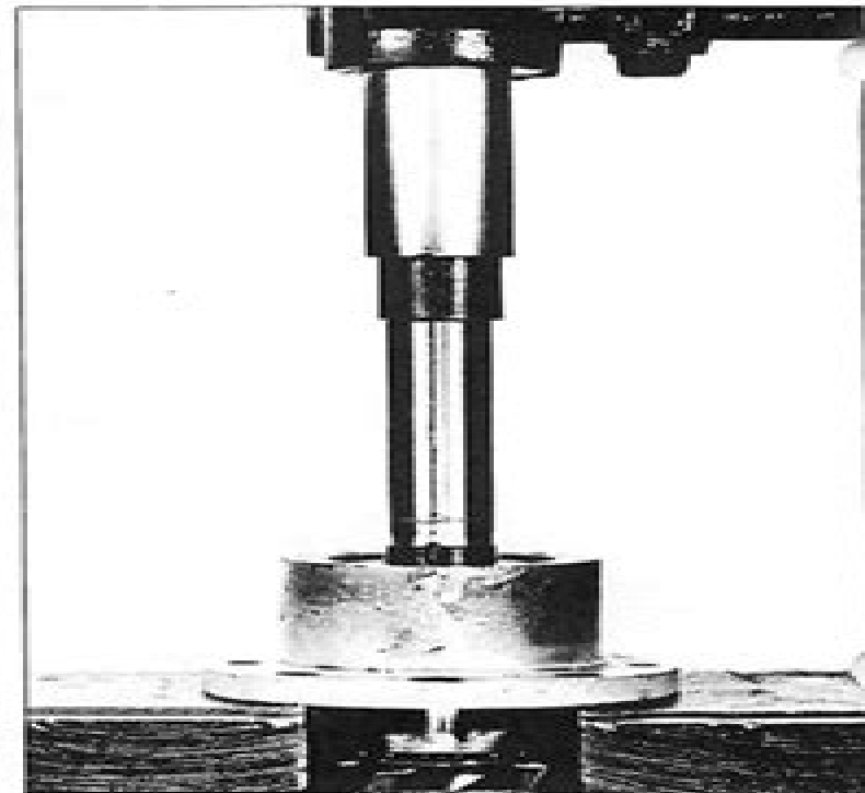
Fig. 5 - Pressing Pinion Shaft from Pinion Bearing
