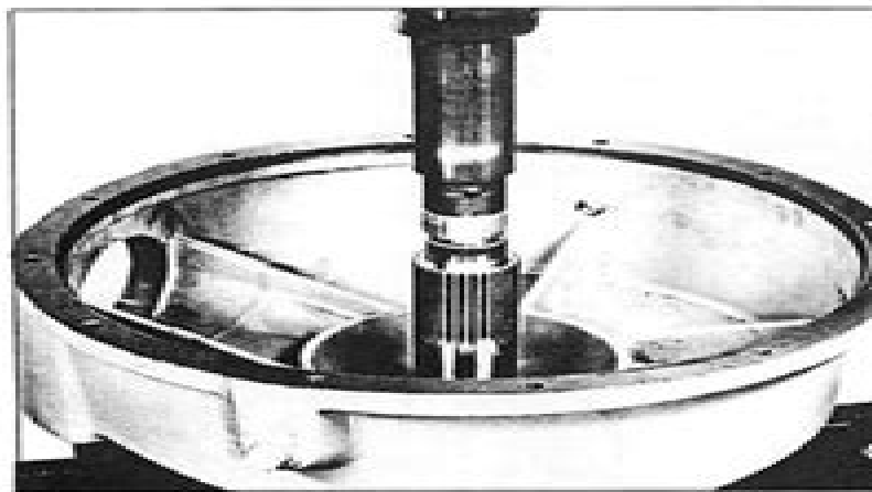
Fig. 4 - Pressing Main Drive Shaft from Gear Housing
