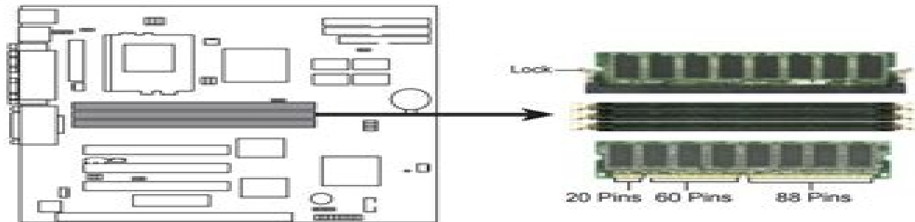
P5-99VM 168-Pin DIMM Sockets
