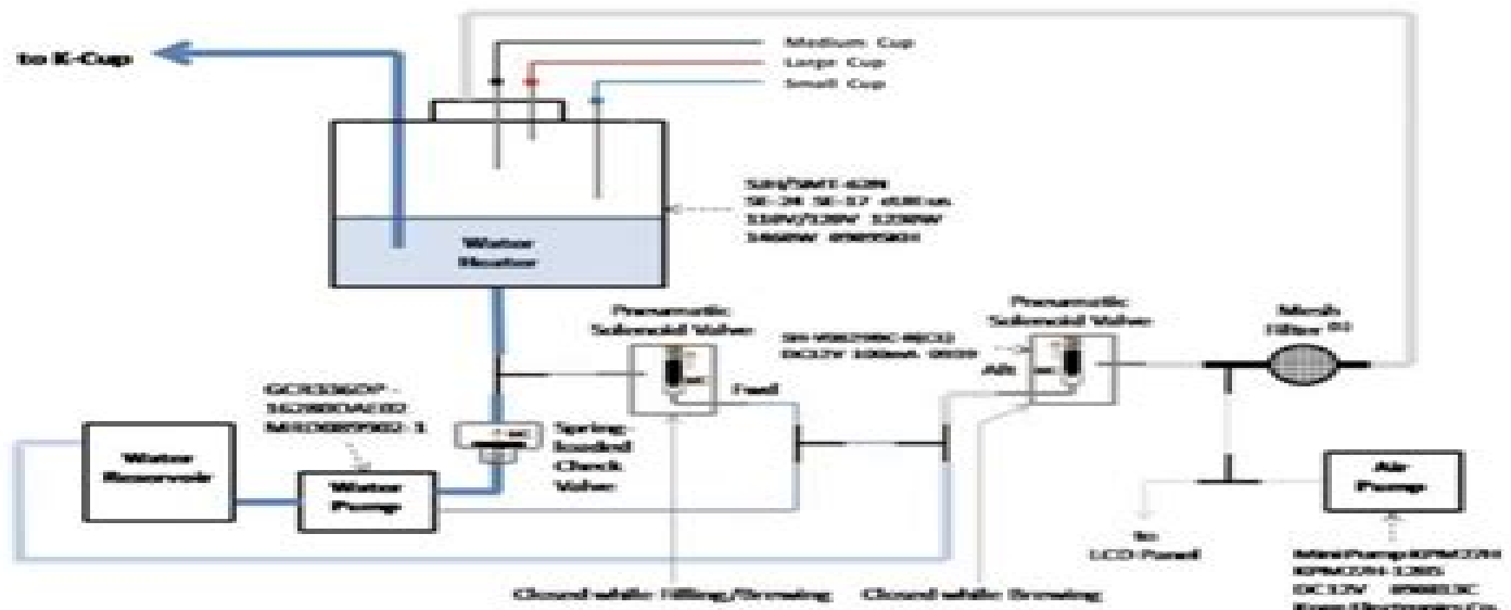
Keurig Mechanical Schematic
