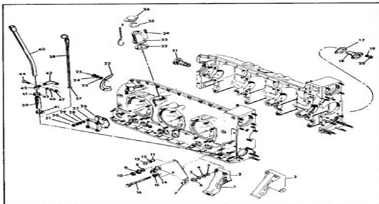
Figure 3. Crankcase Associated Parts.
