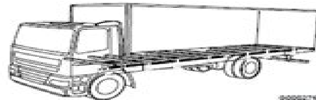
Fixed body with sub-frame, BAM 1
