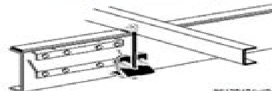
Tie rod mounting, body without sub-frame (with mounting strip)
