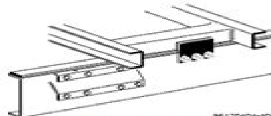
Attachment plate, body without sub-frame (with mounting strip)
