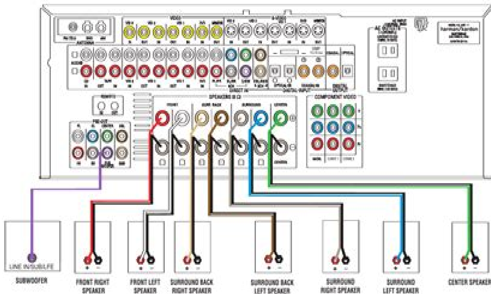
Figure 2 – Speaker Connections
