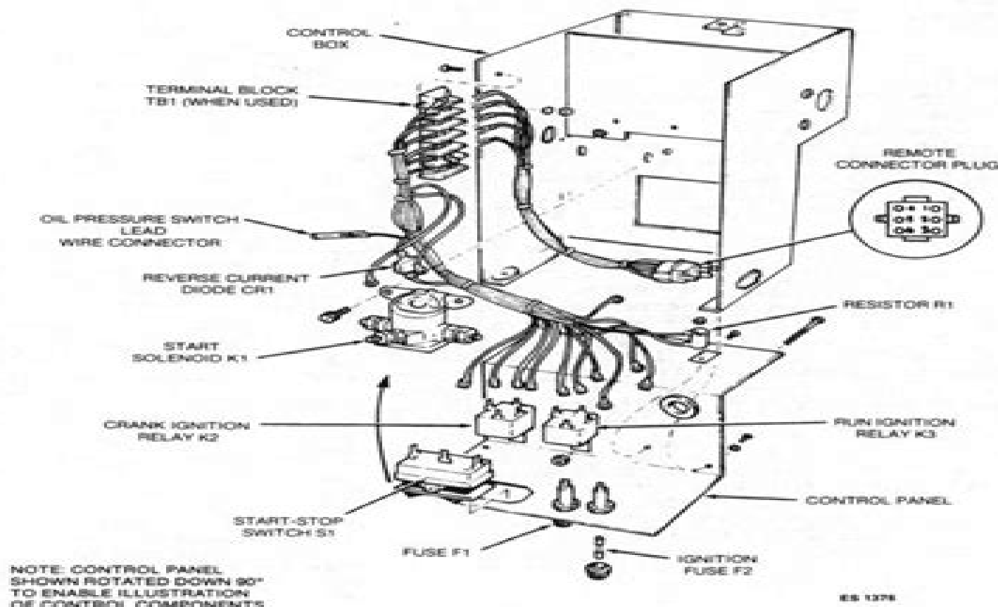
FIGURE 39. BGA, BFA, AND NH (SPEC K-P) CONTROL
