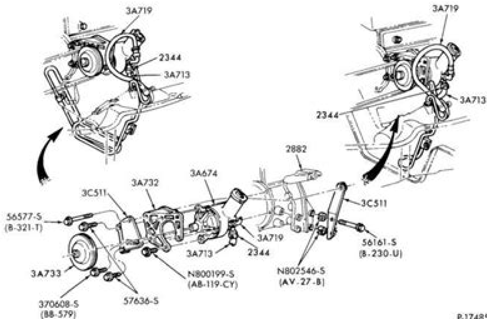
POWER STEERING HOSE and PUMP INSTALLATION 1980/86 F-U100/350 — 6 CYL. 300 (4.9L)
