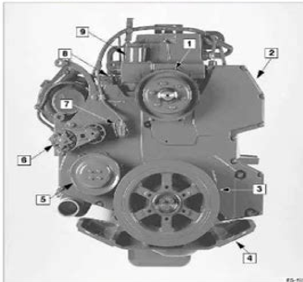
Figure L23 Front View Component Location On Engines Equipped With Chassis Mounted ECM And IDM
