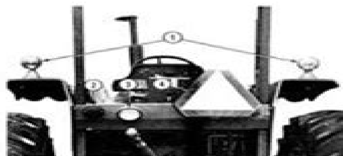
Figure 5 Rear Lights-Tractor Without Cab 1. Flasher/Turn Signal Lights 4. Slow Moving Vehicle (SMV) Emblem 2. Tail Light 3. Rear Work Light
