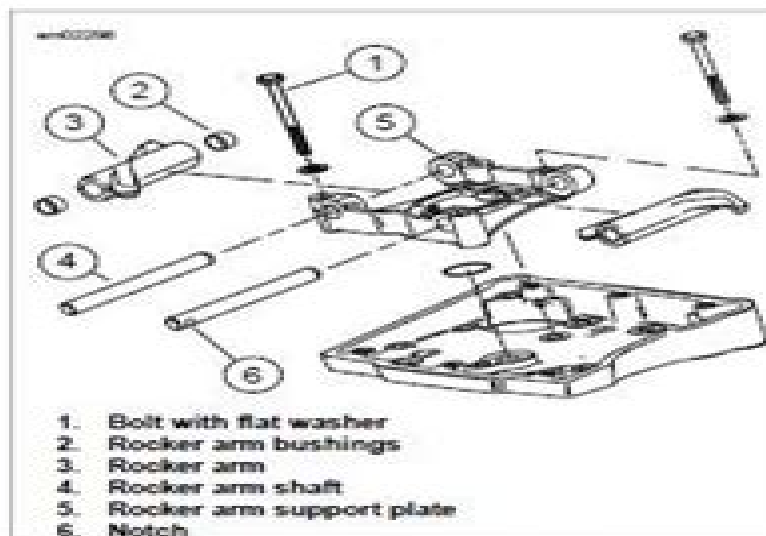
Figure 3-69. Rocker Arm Assembly
