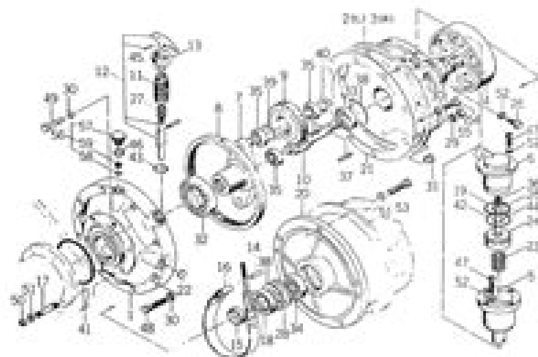
Fig. 4-2-3 Reduction unit
