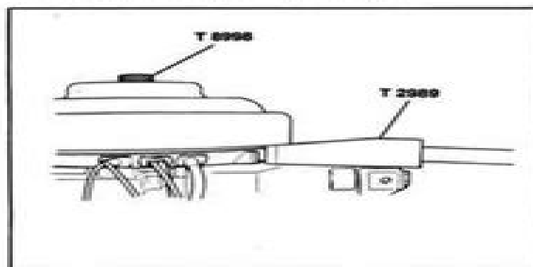
Figure 2. Removing Flywheel.
