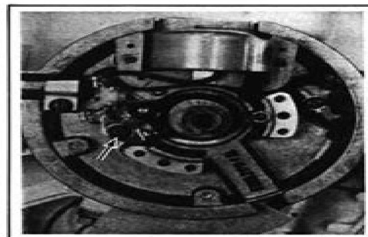
Figure 3. Removing Condenser.
