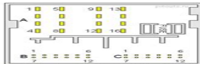
40 (16+12+12) pin QuadLock Fakra Head Unit / Car Stereo connector
