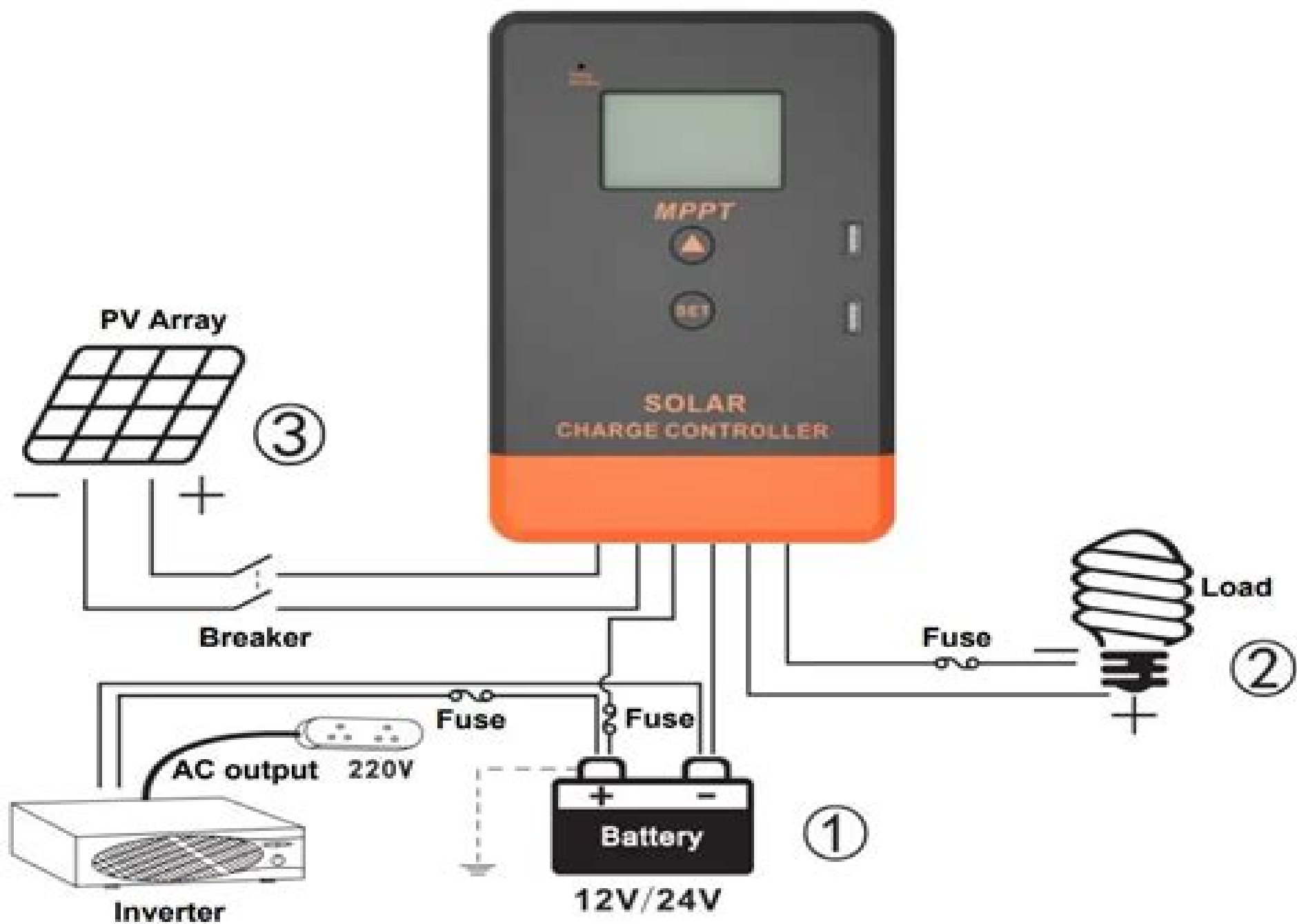
Photo 2 Connection diagram
