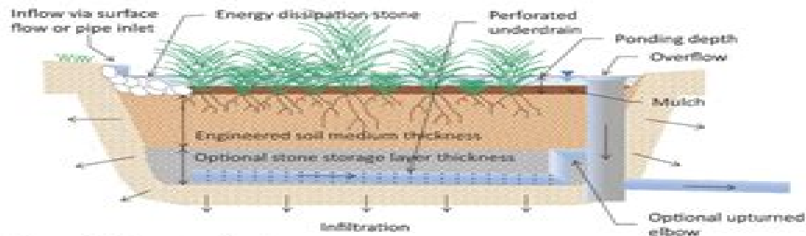
Figure 1. Cross-section view.
