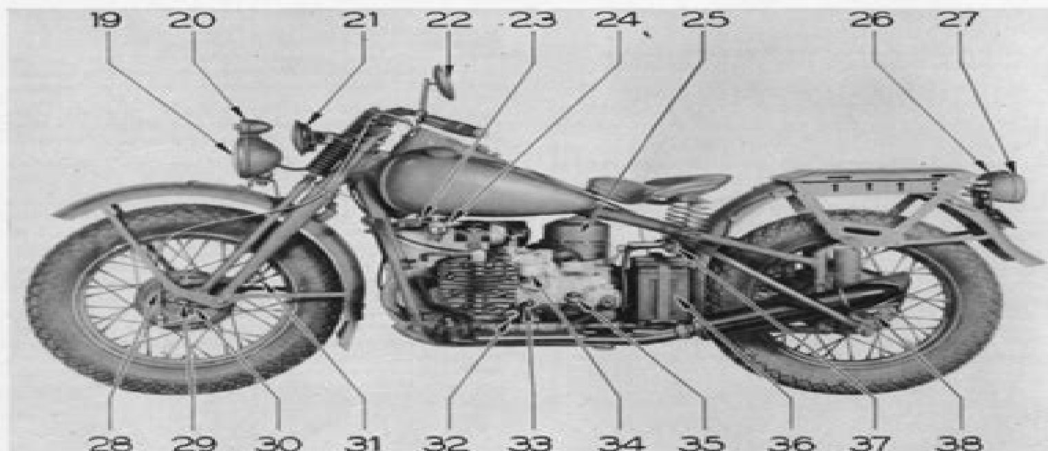
ILLUS. 5—LEFT SIDE VIEW, DETAILS 19 TO 38
