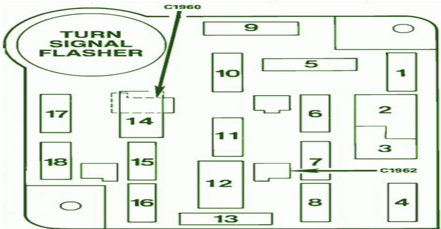
Figure 1 - Fuse Panel
