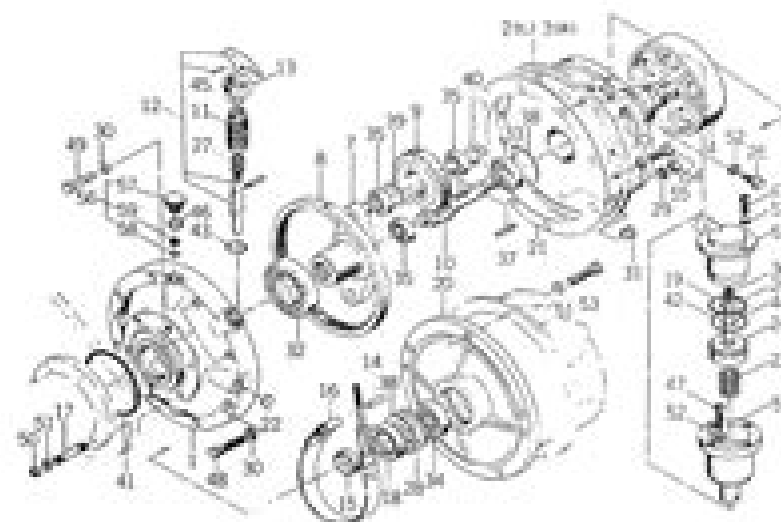
Fig. 4-2-3 Reduction assembly
