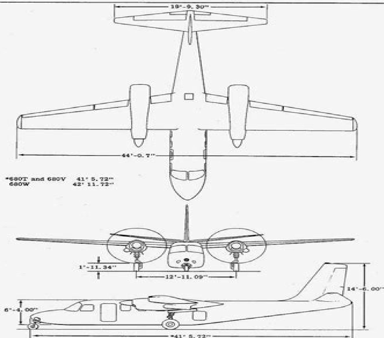
Figure 1-2. General Dimensions
