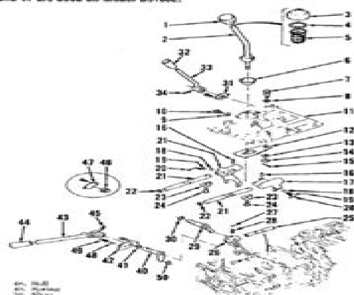
Fig. 73—Exploded view of shifter mechanism used on Models 851000 and 851006. Components 33 through 44 are used on Model 851000 and components 46 and 47 are used on Model 851006.
