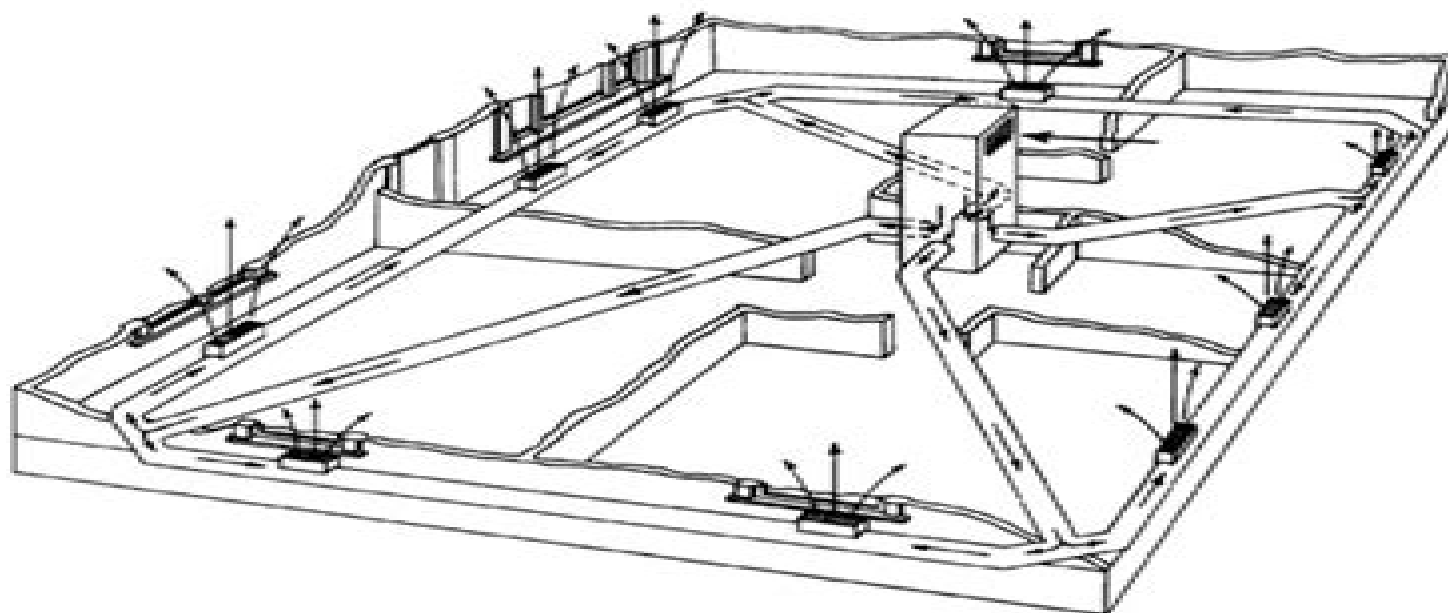
Figure 6-4. Perimeter loop delivery system.
