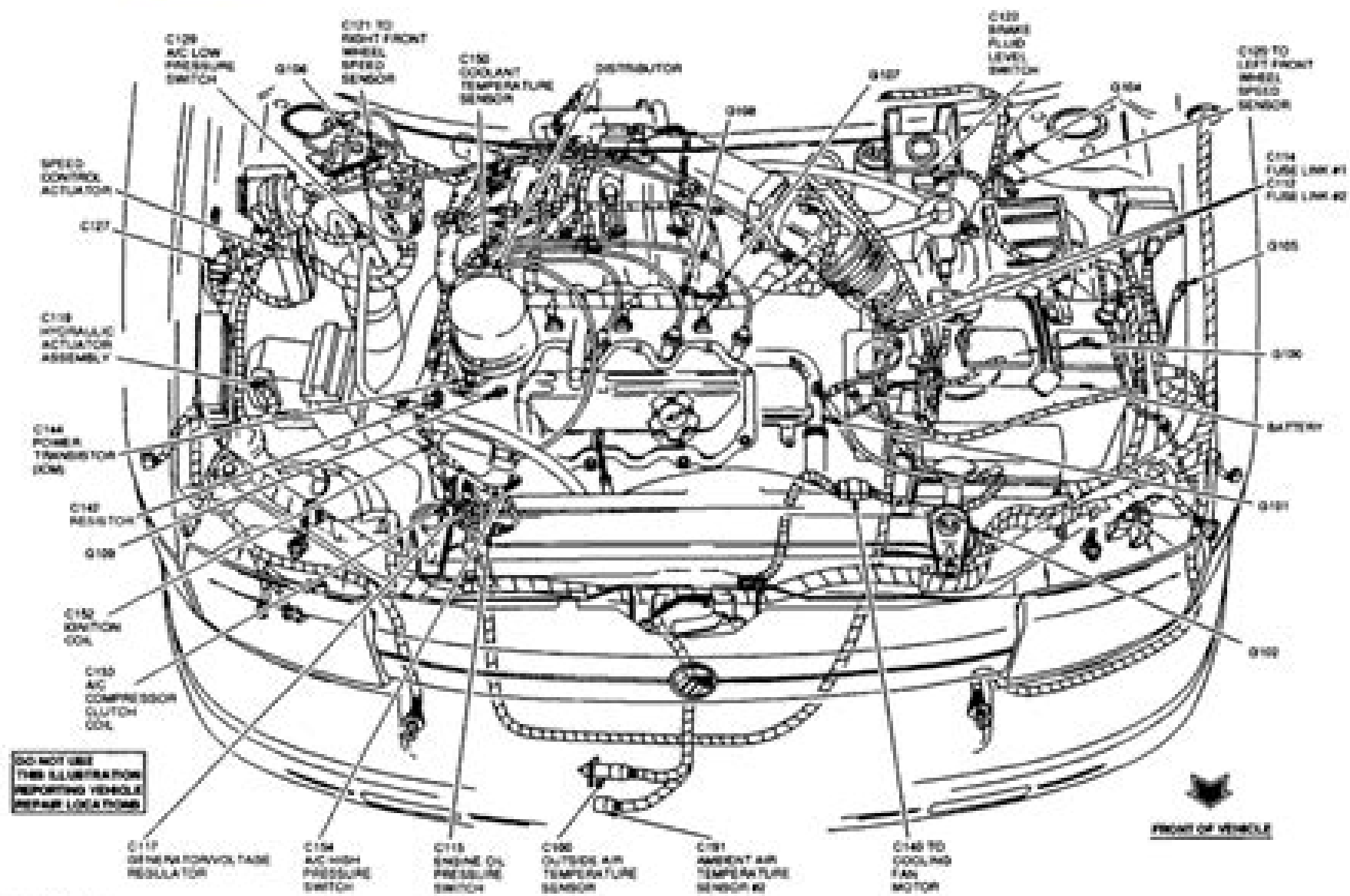
Fig 5: Locating Fusible Links
