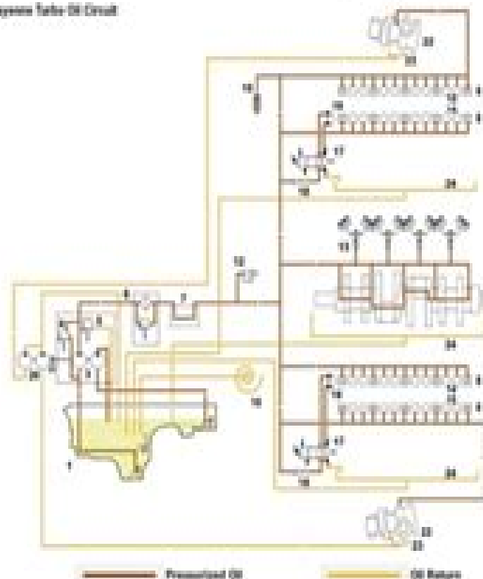
Cayenne Turbo Oil Circuit
