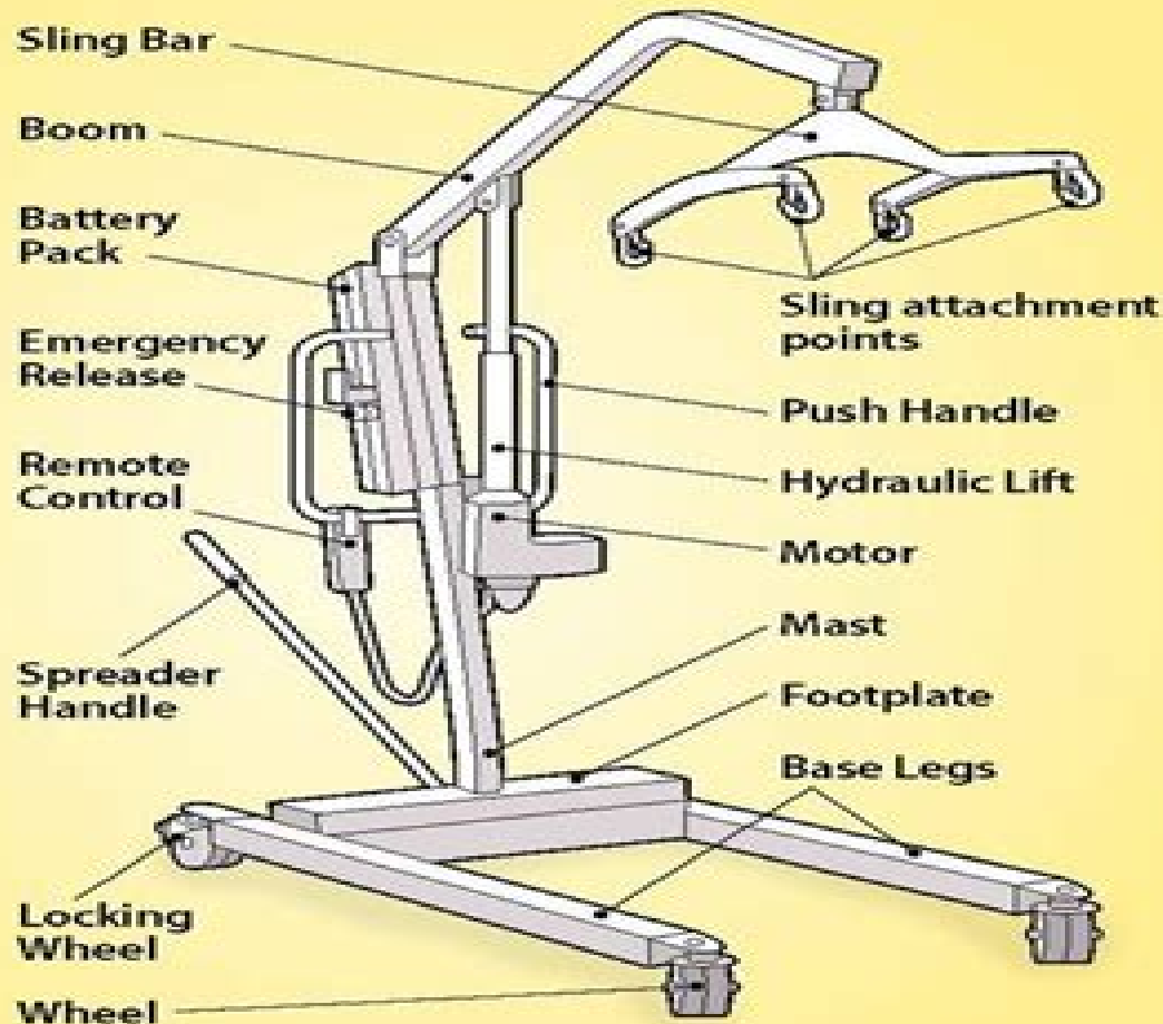
Floor-Based, Full-Body Sling Lift
