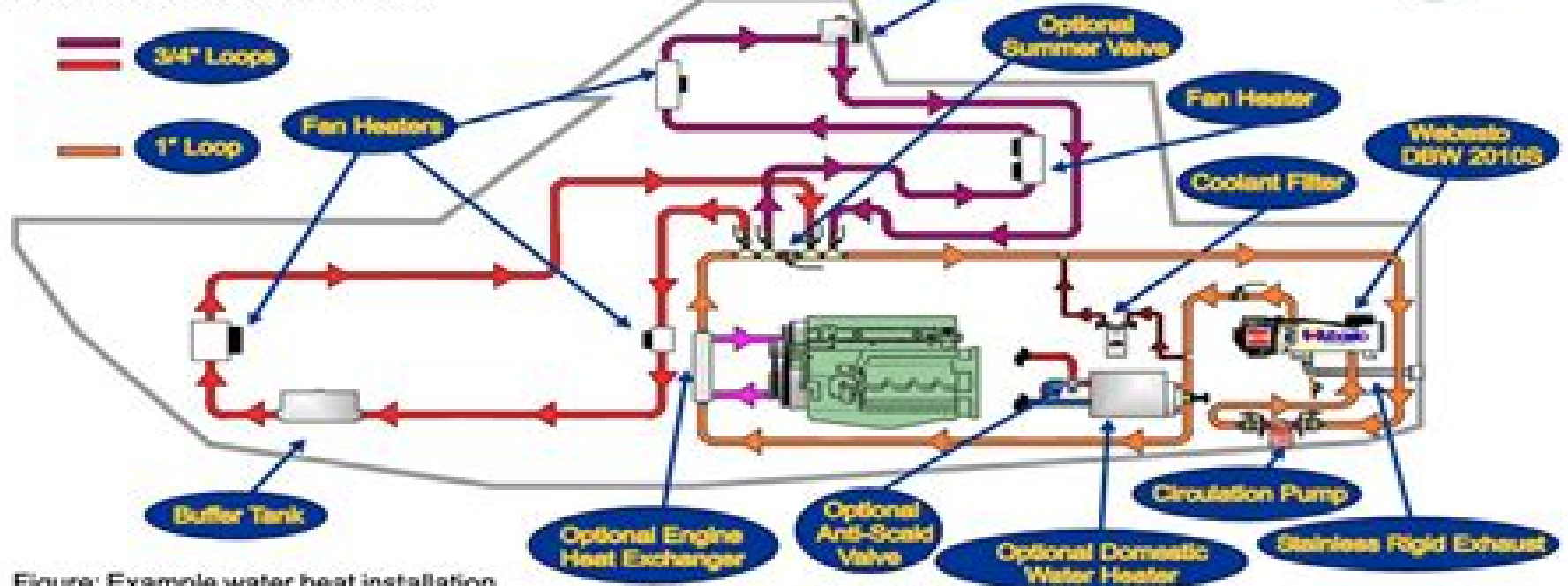
Figure: Example water heat installation. See manual for installation guidelines.
