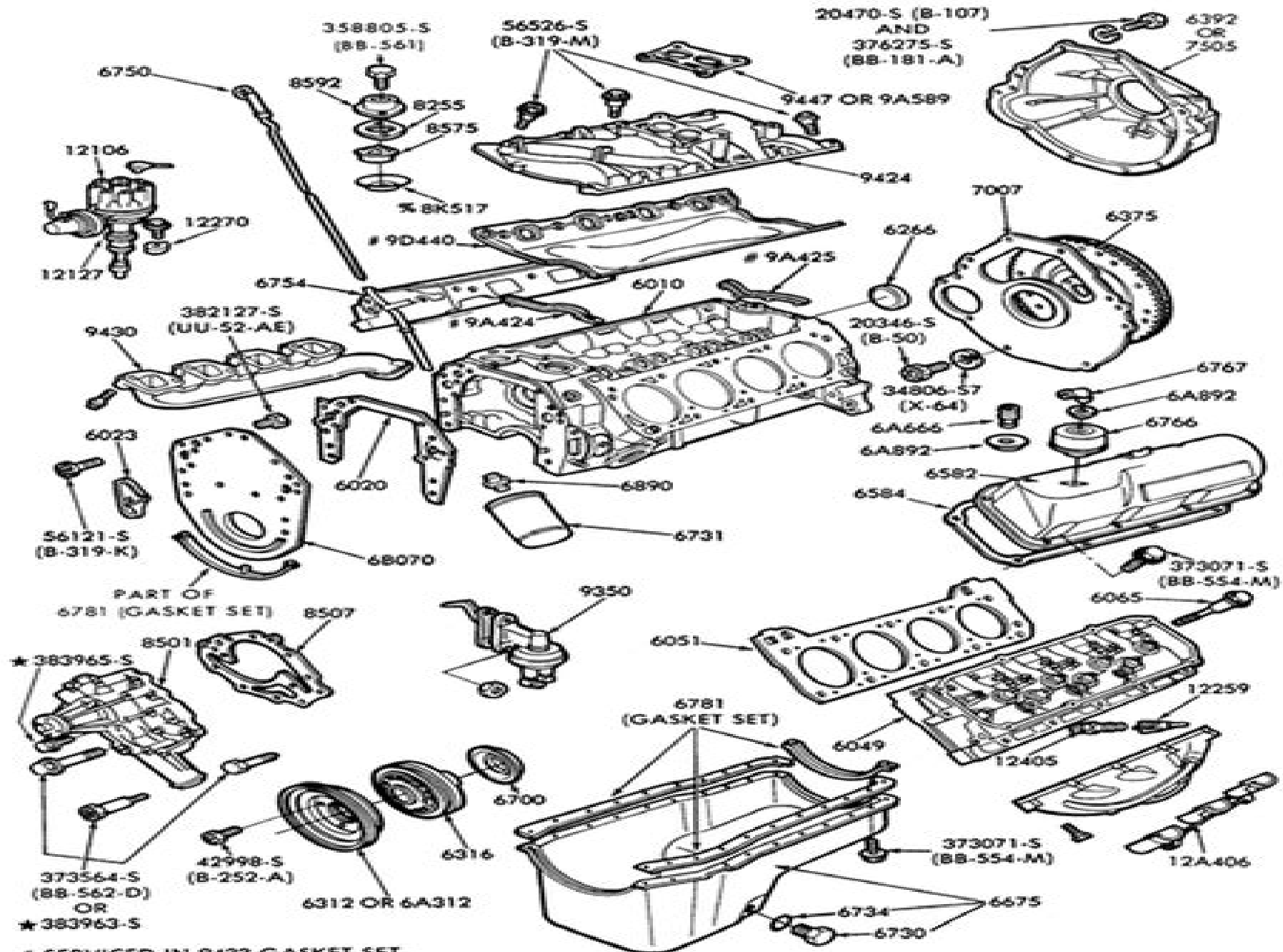
CYLINDER BLOCK and RELATED PARTS (EXTERNAL) — TYPICAL 1980/82 8 CYL. 351M (5.8L) and 400 (6.6L)
