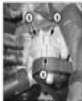
1-13a The mark (1) on the upper battery terminal must remain between the clamps (2) on the terminal mount (2) always, even here.
