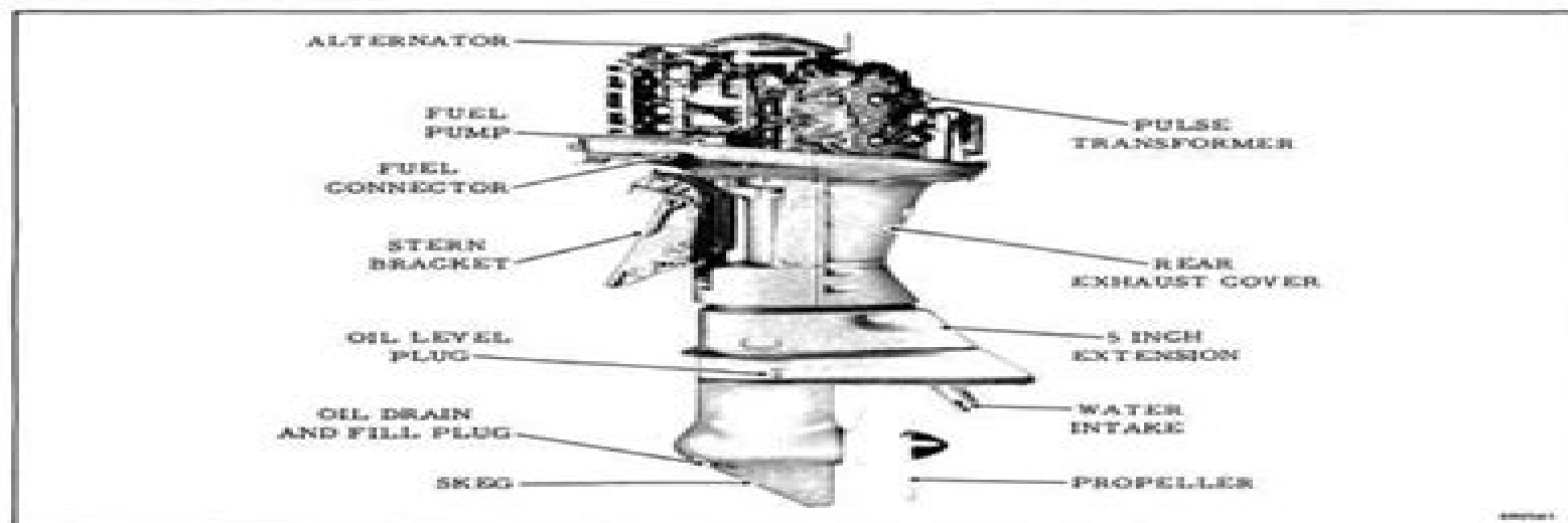
Figure 1-2. Port Side
