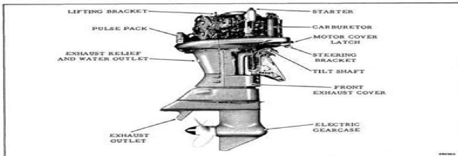
Figure 1-1. Starboard Side
