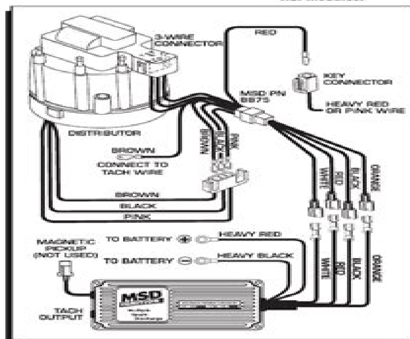
Figure 2 Wiring the PN 8875 Harness
