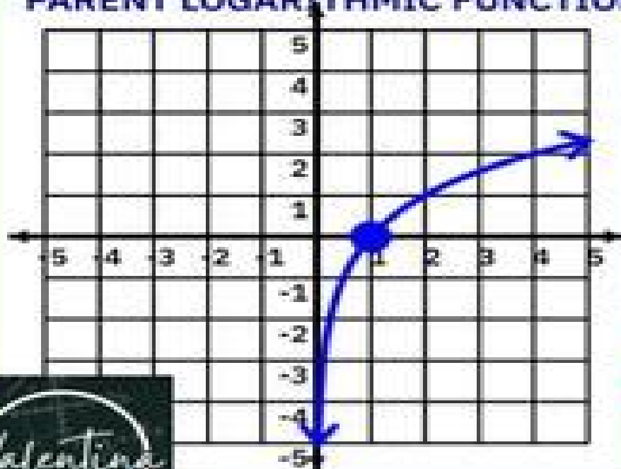
PARENT LOGARITHMIC FUNCTION
