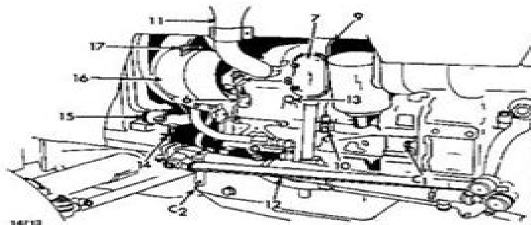
FIG. A.O/S LEFT SIDE VIEW OF ENGINE INSTALLED
