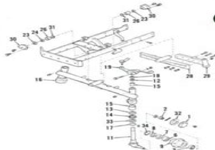
Fig. 3—Exploded view of fixed thread front axle (18) used on 1300 and 1500 models. Axle center member (28) and extensions (29) are used on 1200, 1310, 1500 and 1510 adjustable axle models.
