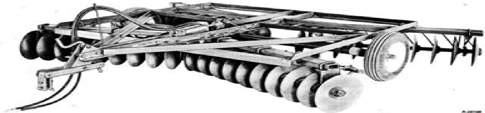
37 Wheel-Controlled Disk Harrow with remote control hydraulic cylinder, scrapers, and weight box.
