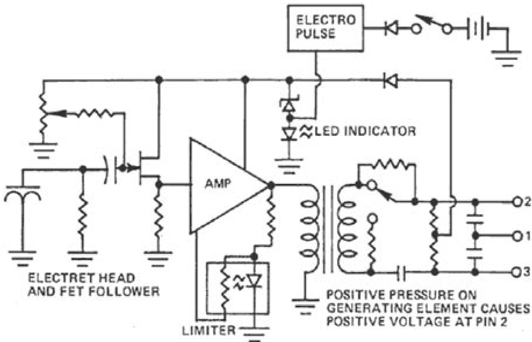
FIGURE 5 — Circuit Block Diagram
