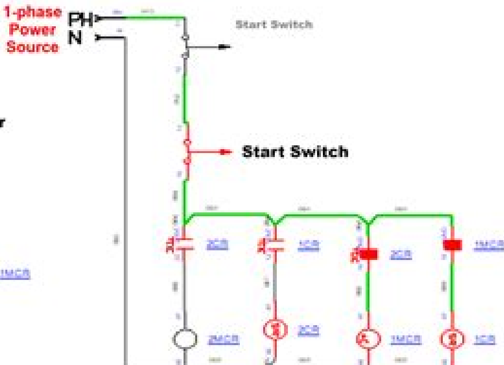
CONTROL CIRCUIT
