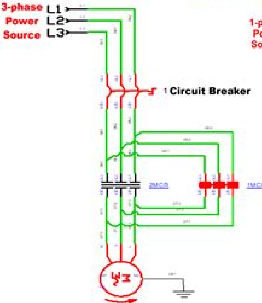
POWER CIRCUIT
